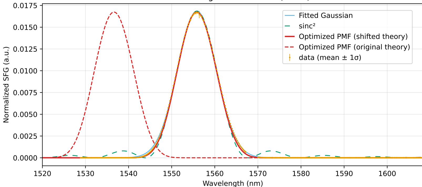
Four-step BG-removed Normalized SFG vs Wavelength (C+L) Shifted & original CPKTP PMF (linear)
